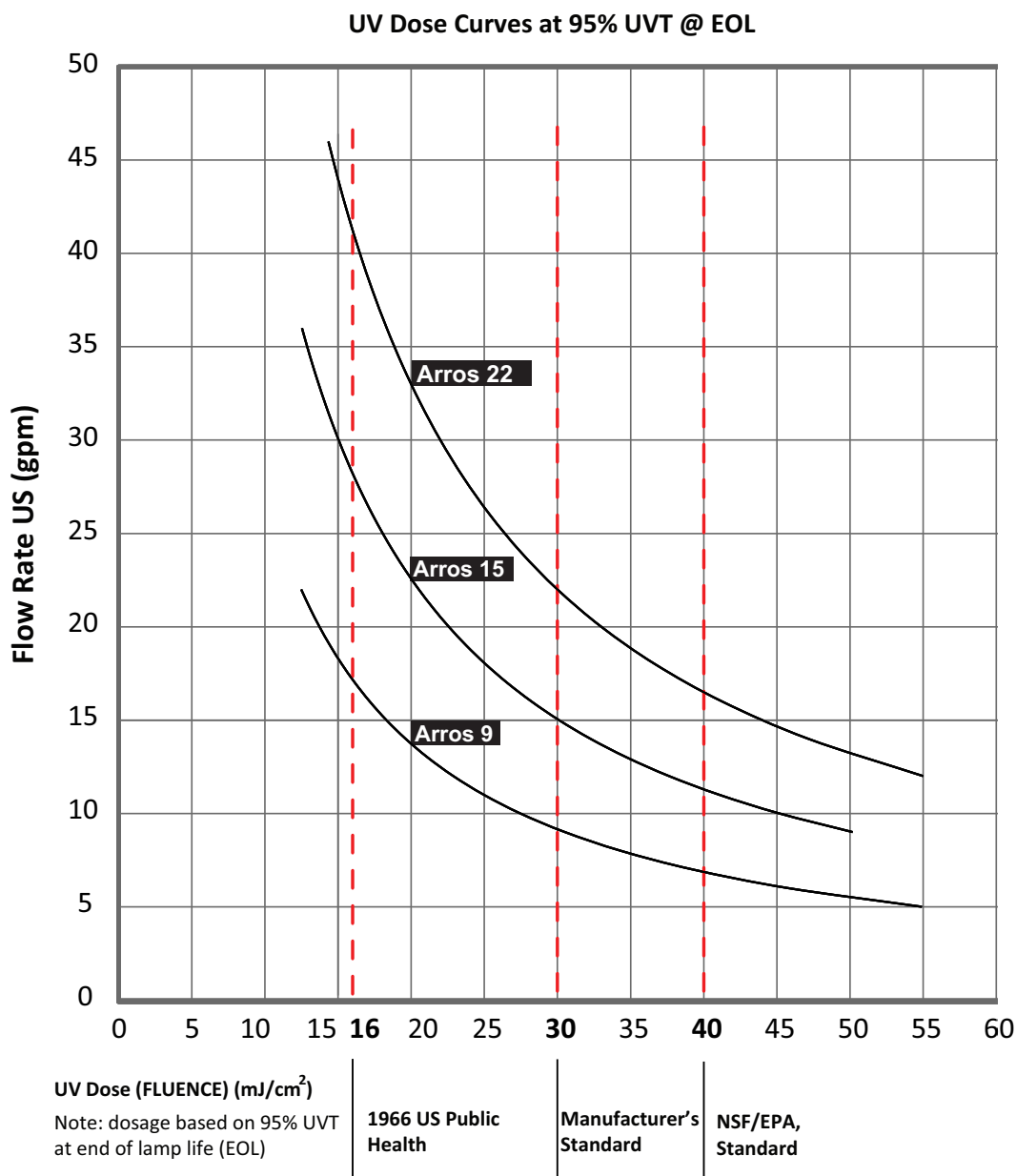
Figure 13 Dose Flow Chart
