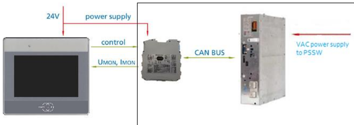
1 to 8x Control Interface+ PSSW powersupply can be connected
