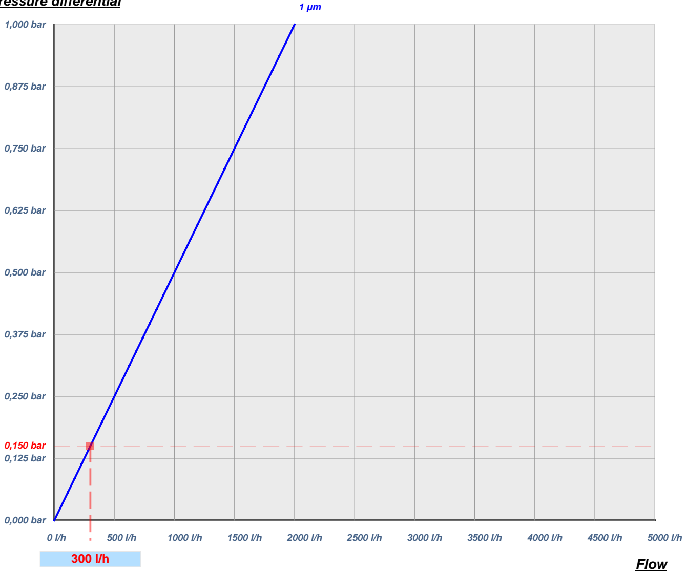
FLOW RATE VS PRESSURE DIFFERENTIAL
