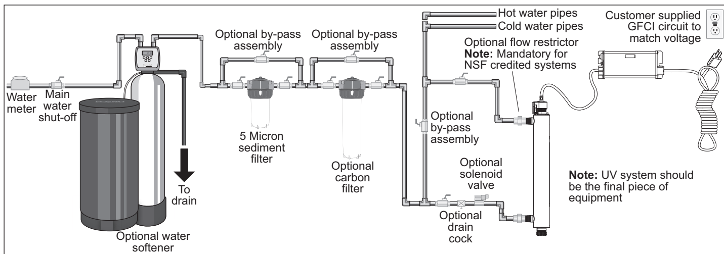
Figure 3 UV System
