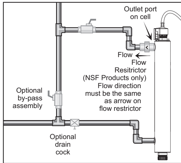
Figure 5 Flow Restrictor
